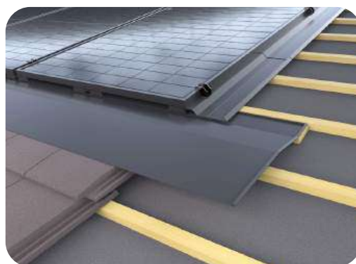
Lower Rigid Flashing
