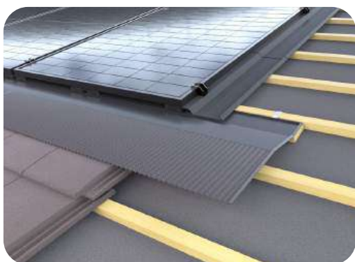
Lower Semi-Rigid Flashing
