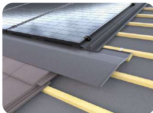
Flashing Strip
