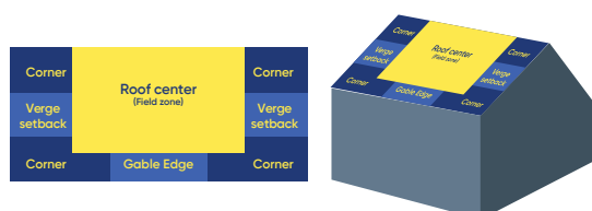
DUAL-PITCH ROOF
