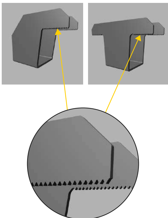
The clamp teeth must bite into the module frame
