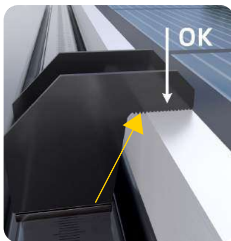
The clamp teeth must bite into the module frame
