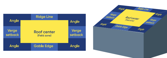
MONO-PITCH ROOF
